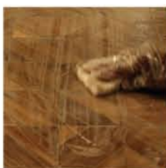
Step-10: Clean excess grout from wood surface
